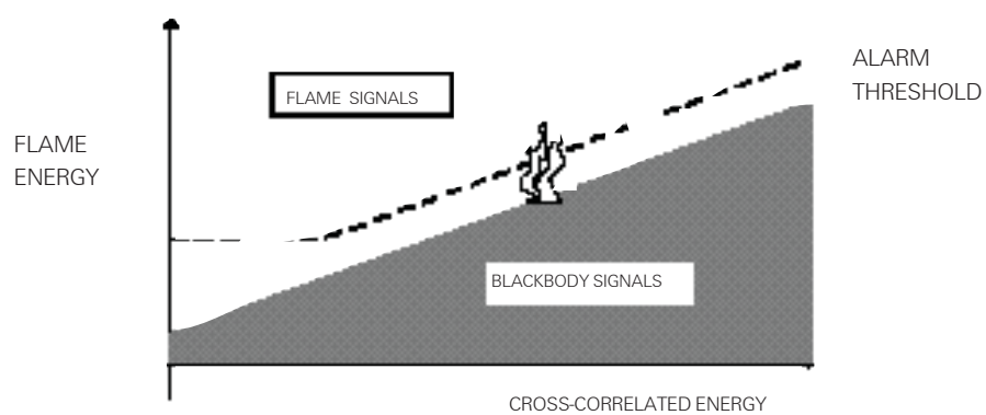
fig. 4. Variable Alarm Threshold
