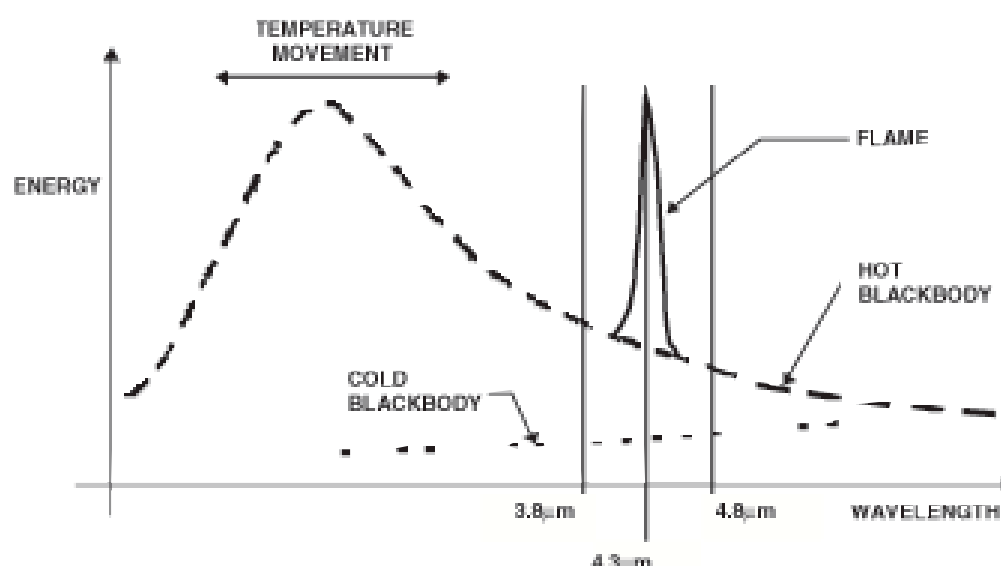
Fig. 3. Blackbody Rejection
