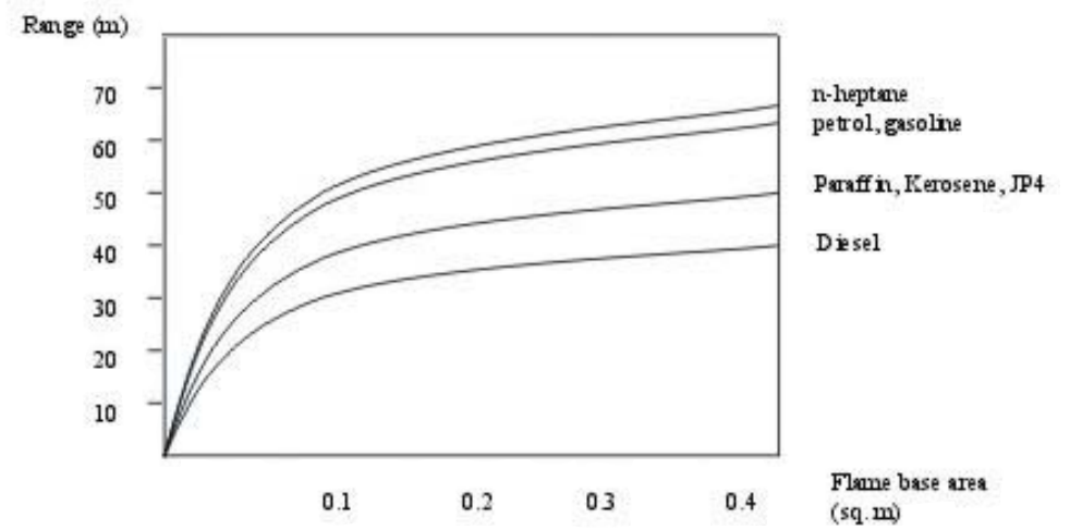
Fig. 1 - Fire Range Test Data
