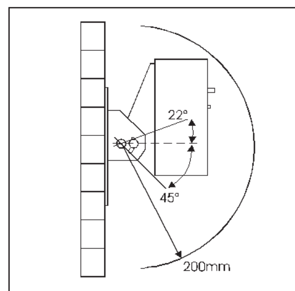
Fig. 5 S200 Mounting Bracket
